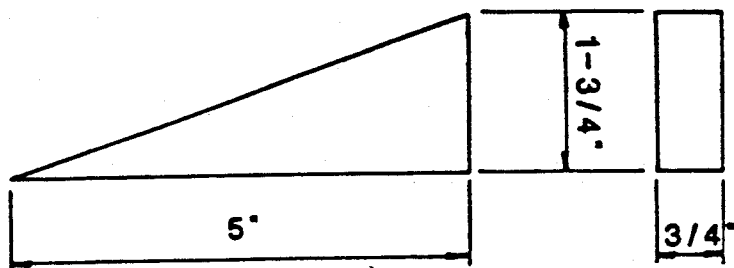
Wedge (2 Req'd per anchor)
