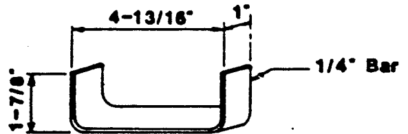
AA2S Alloy Male Hook
