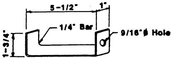
AA3S Alloy Male Hook
