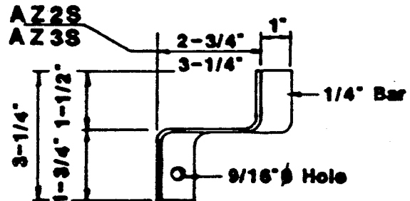
AZ2S Alloy Z-Clip AZ3S Alloy Z-Clip
