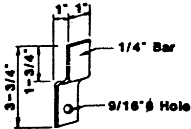
A150S Alloy Clip
