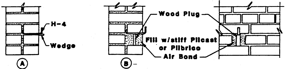
Anchor installation in existing brick wall w/wood plug
