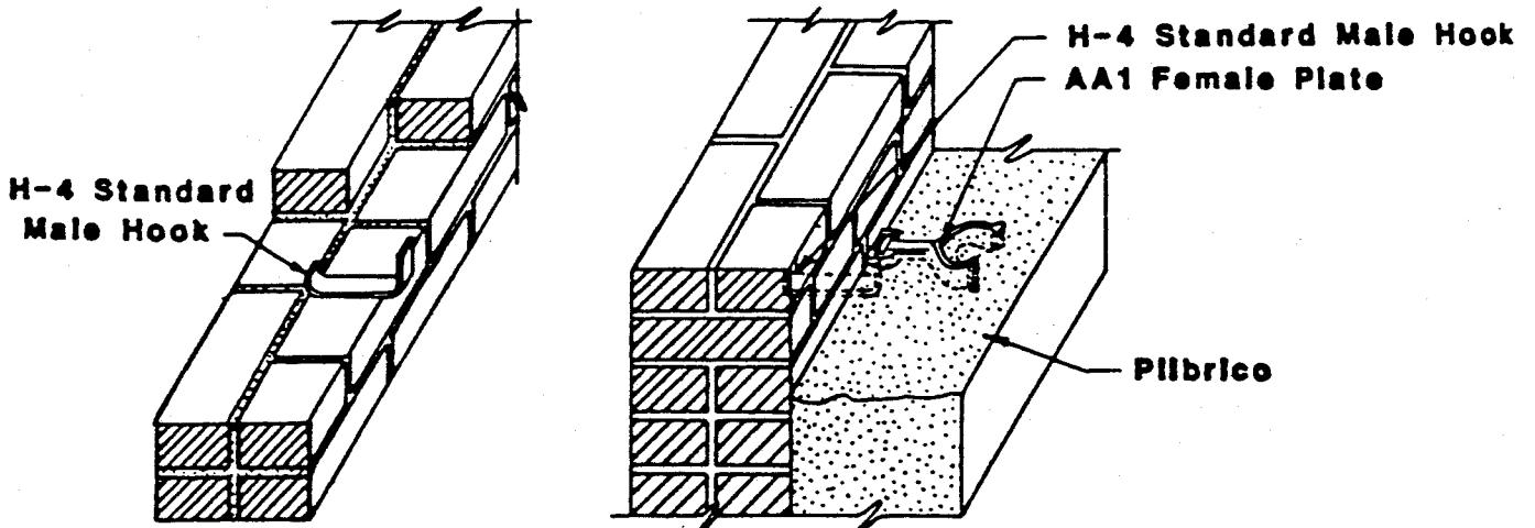
Anchor installation in new common brick walls
