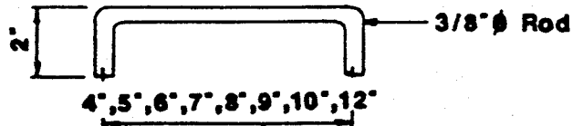
Alloy Pilcast Hooks (Special Lengths Available on Request) 304 S.S.
