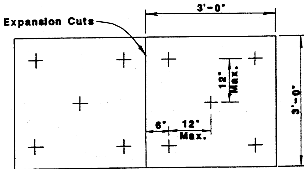
AH-9S Spacings for Plastic Refractory Lining
