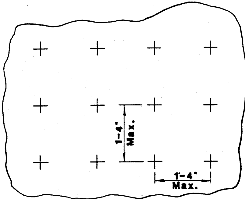
AH-9S Spacings for Castable Refractory Lining
