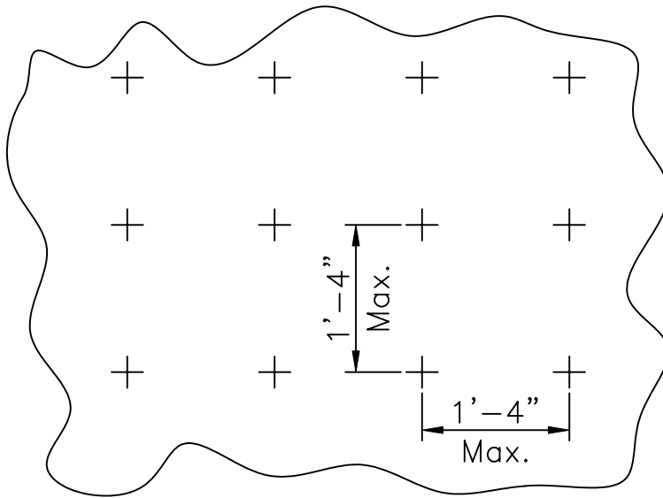
AH-9S Spacings for Castable Refractory Lining
