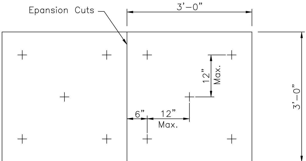
AH-9S Spacings for Plastic Refractory Lining
