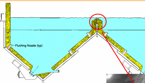
Stainless Steel Cricket Being Added To Existing Wet-Bottom Ash Hopper
